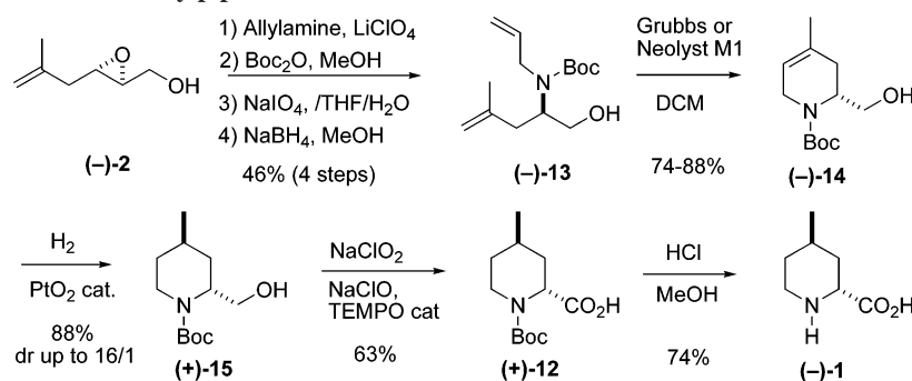
SCHEME 4. Synthesis of trans -4-Methylpiperolic Acid 1
