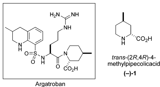
FIGURE 1. Structures of Argatroban and trans -(2 R ,4 R )-4-methylpipercolic acid.
